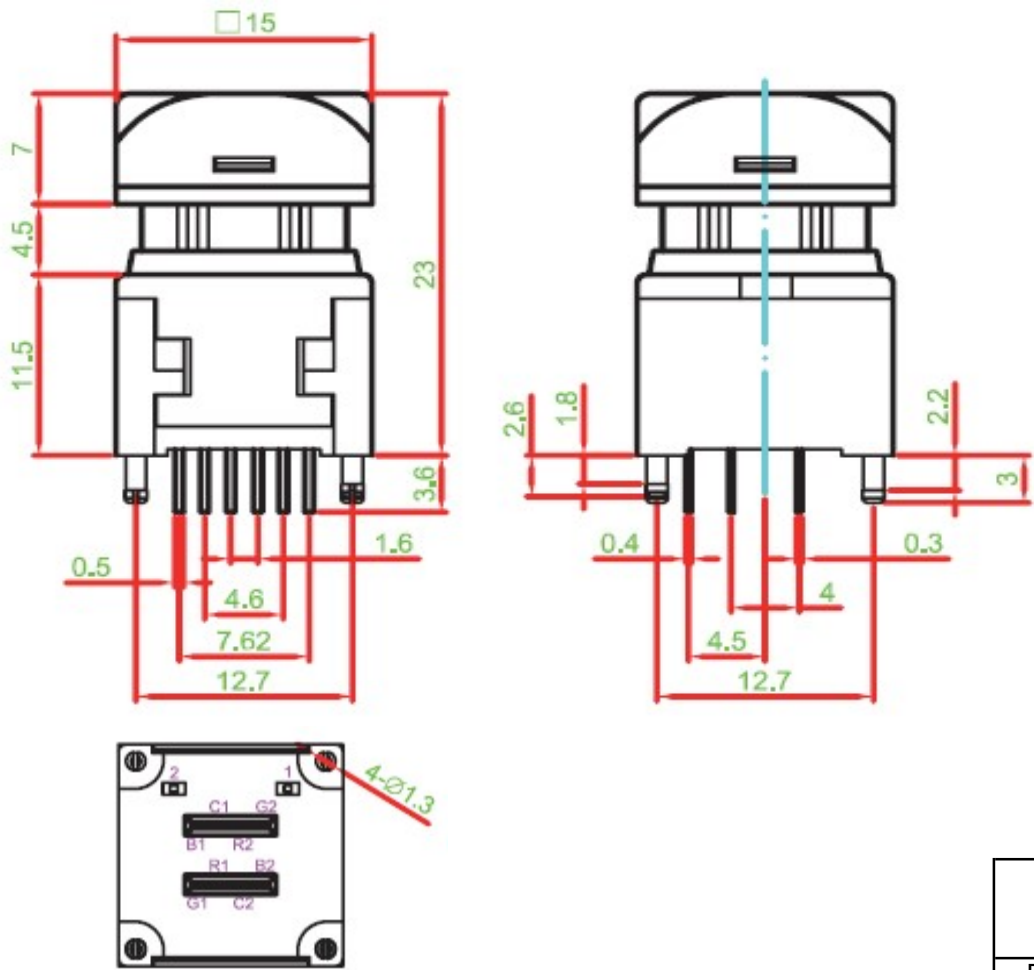
Technical Dimensions ( mm)
