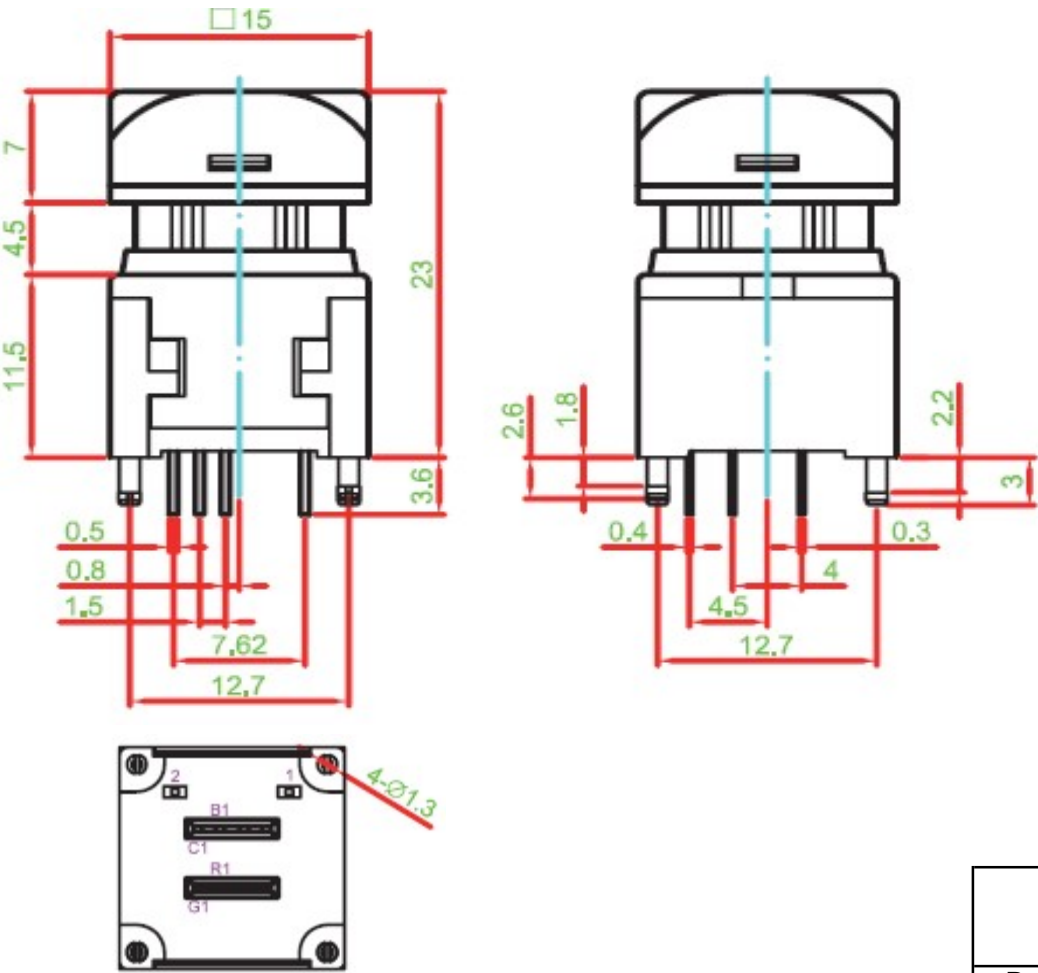
THT Panel Tact Switch 15x15mm H=23mm
