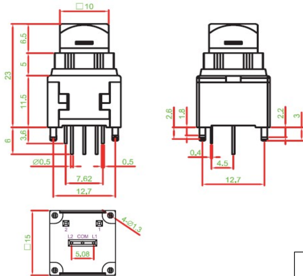
THT Panel Tact Switch 10x10mm H=23mm
