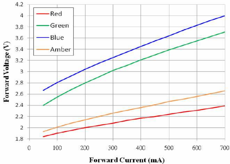
Typical Forward Current Characteristics
