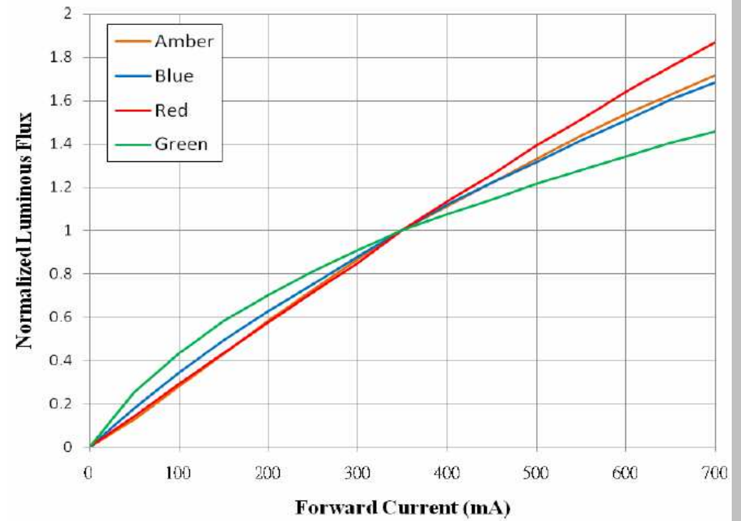
Typical Light Output Characteristics over Forward Current
