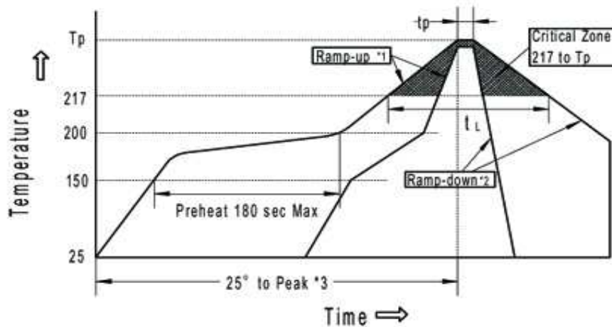
Reflow Profile
