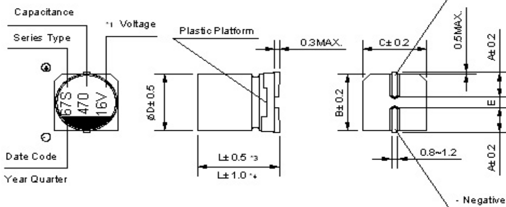
Dimension of Size Ø 8x10,5 ~ 16mm
