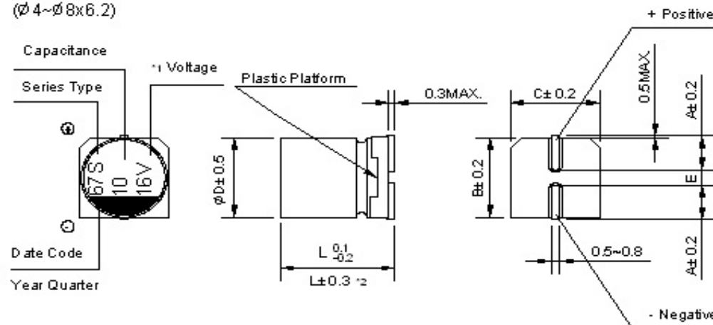
Dimension of Size Ø 4~ 8x6,2mm
