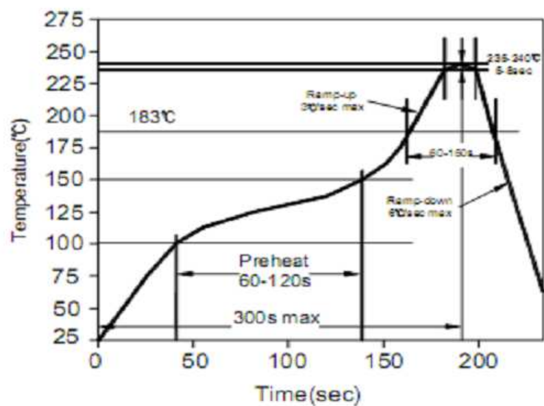
Classification Reflow Profile (JEDEC J-STD-020C)
