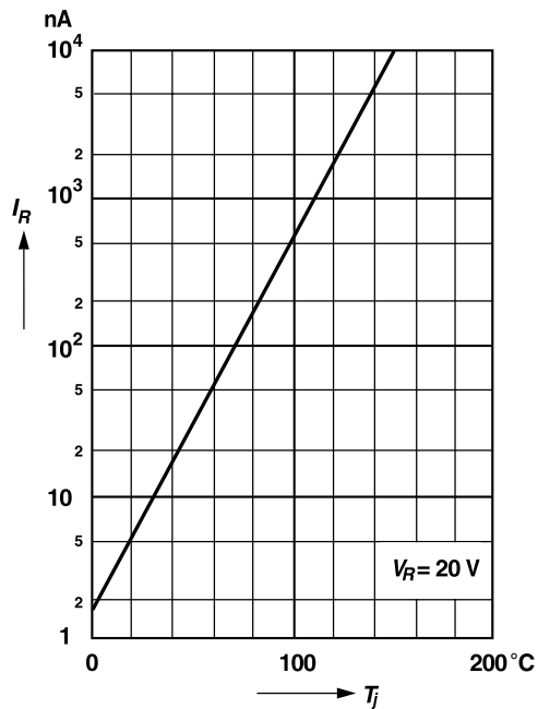
FIG 5 Leakage Current Versus Junction Temperature
