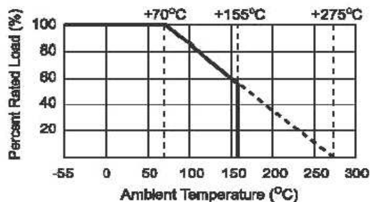
Derating Curve
