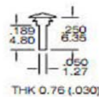
PCB Terminal Option (B)
