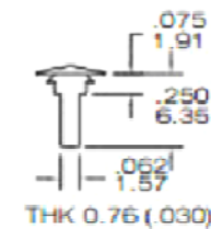
PCB Terminal Option (B)
