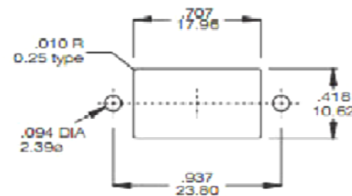
Panel Mounting Dimension
