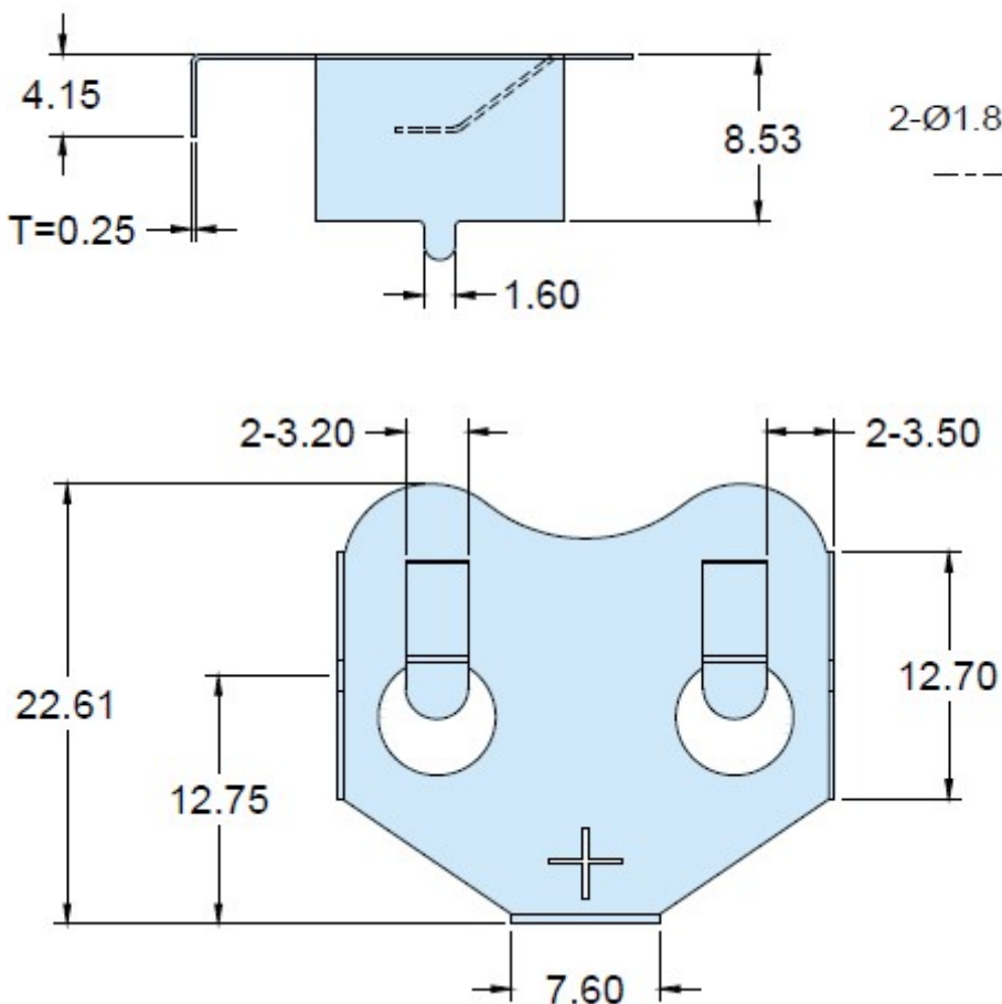
Technical Drawing (mm)
