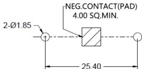
PCB-PAD-Layout (mm)
