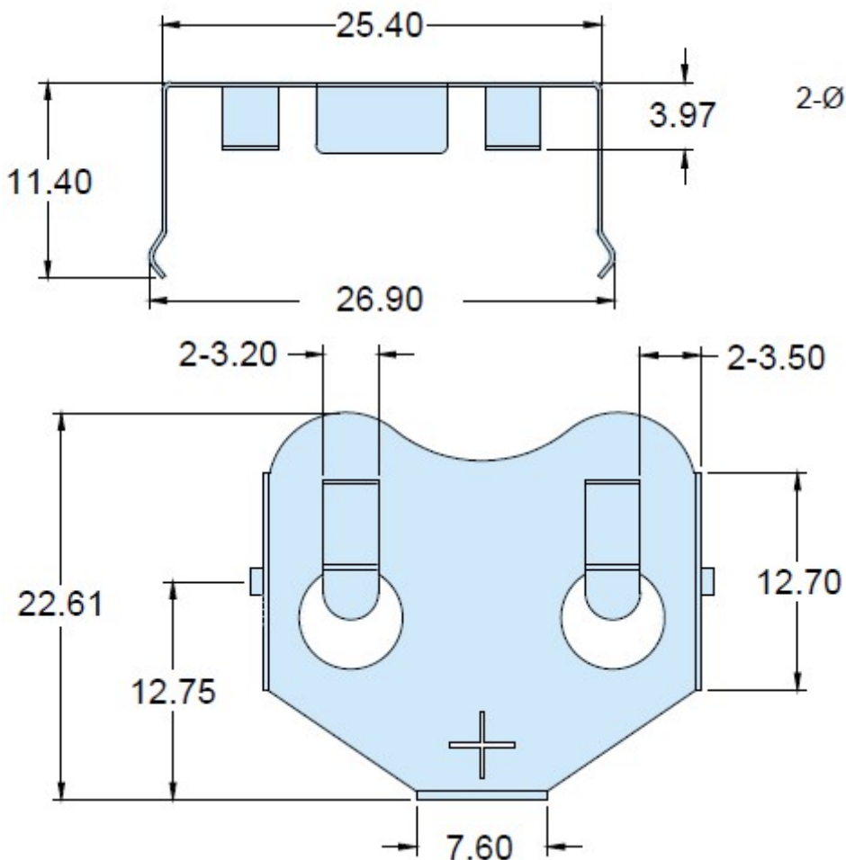
Technical Drawing (mm)
