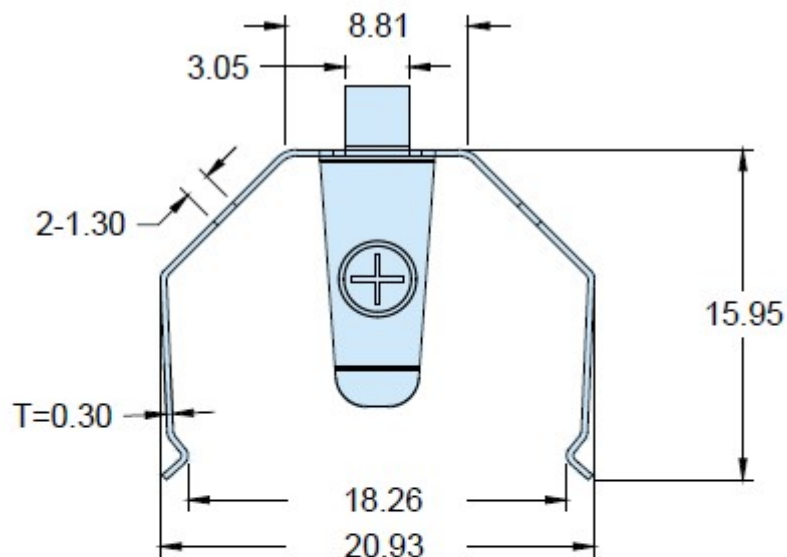
Technical Drawing (mm)
