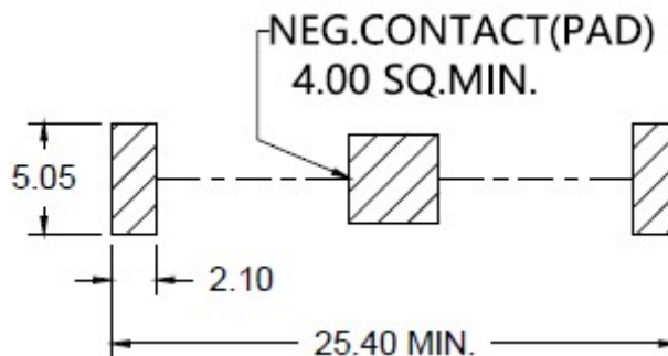
PCB-PAD-Layout (mm)
