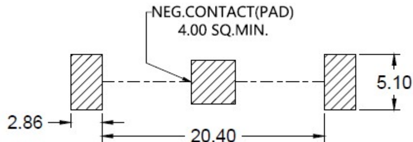
PCB-PAD-Layout (mm)
