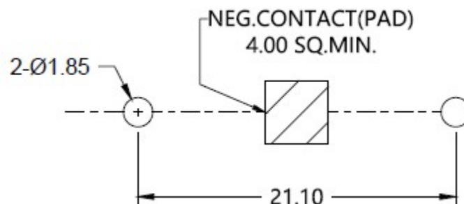
PCB-PAD-Layout (mm)
