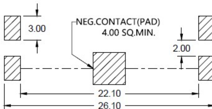
PCB-PAD-Layout (mm)
