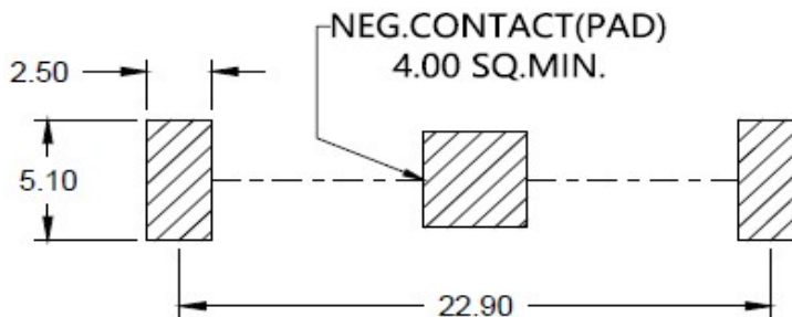
PCB-PAD-Layout (mm)
