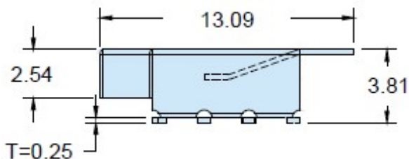
Technical Drawing (mm)
