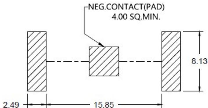
PCB-PAD-Layout (mm)
