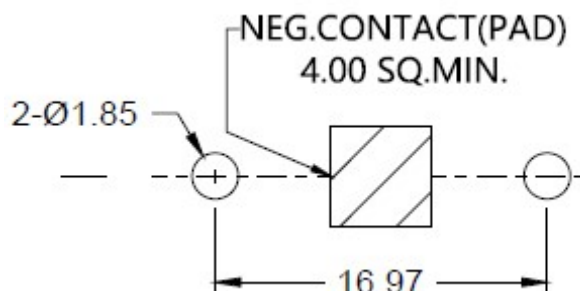
PCB-PAD-Layout (mm)
