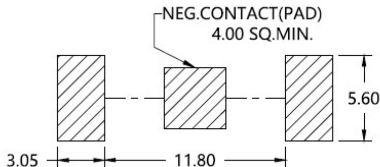
PCB-PAD-Layout (mm)
