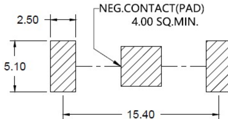
PCB-PAD-Layout (mm)
