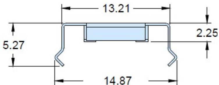
Technical Drawing (mm)
