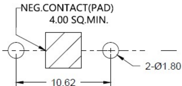
PCB-PAD-Layout (mm)
