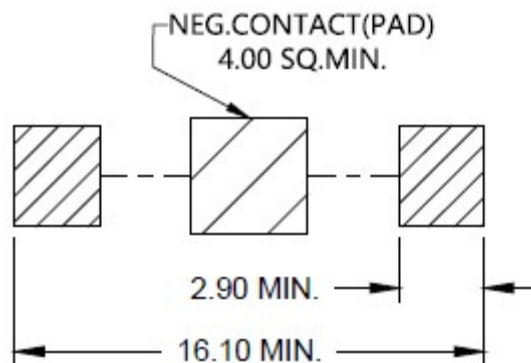
PCB-PAD-Layout (mm)
