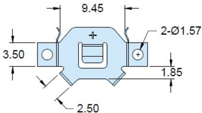
Technical Drawing (mm)
