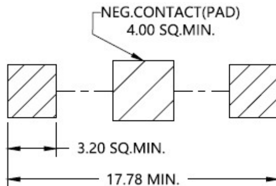
PCB-PAD-Layout (mm)
