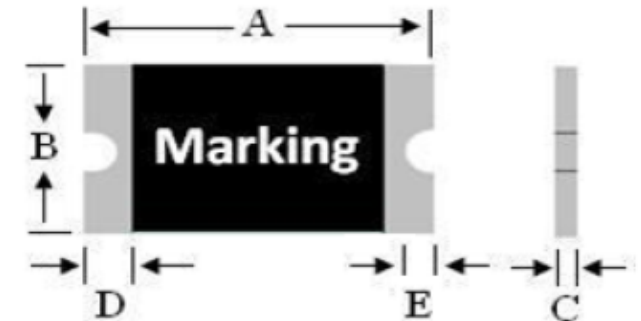
Dimensions (mm)
