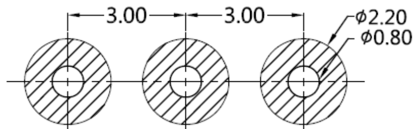
PCB Layout ( mm)
