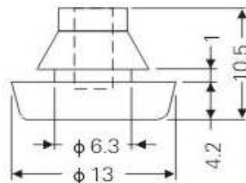
MOUNTING HOLE \phi 6.35
