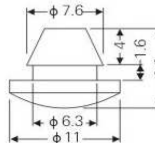
MOUNTING HOLE \phi 6.5
