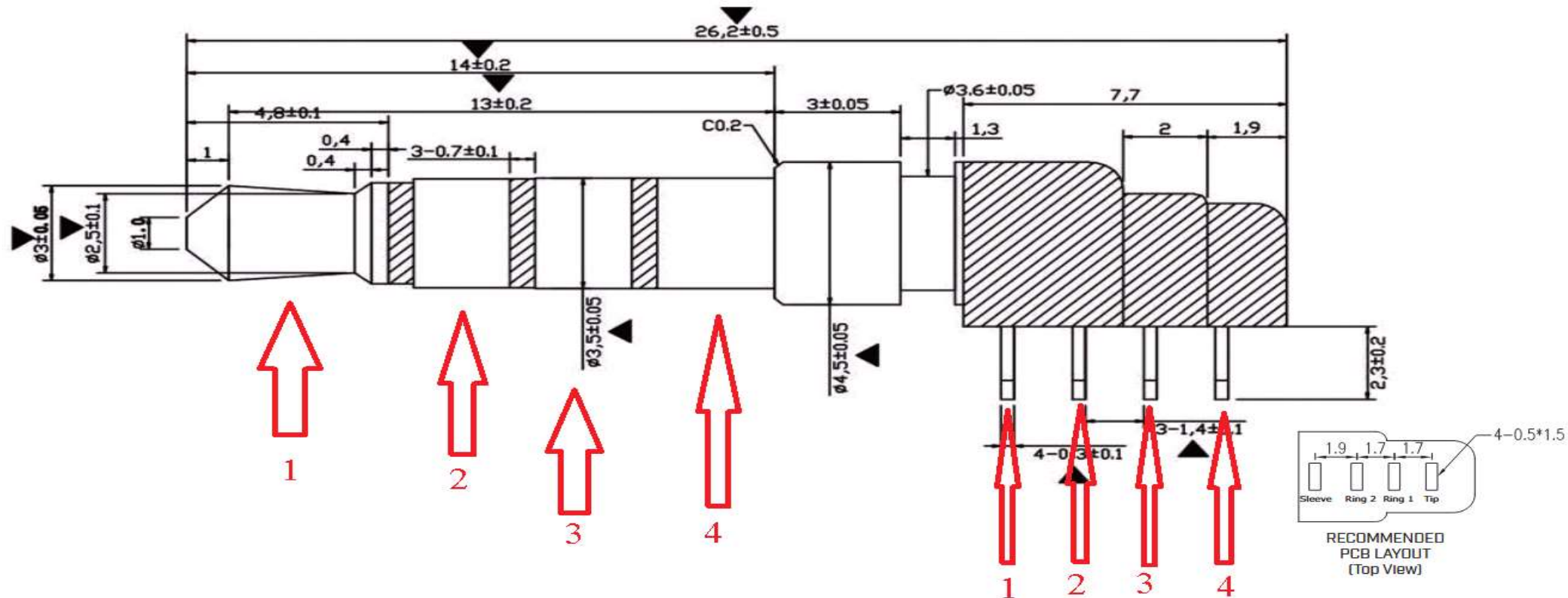
Drawing ( dimensions all into mm)
