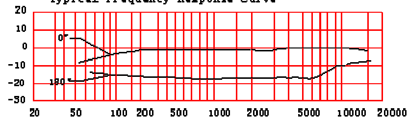
Typical Frequency Response Curve
