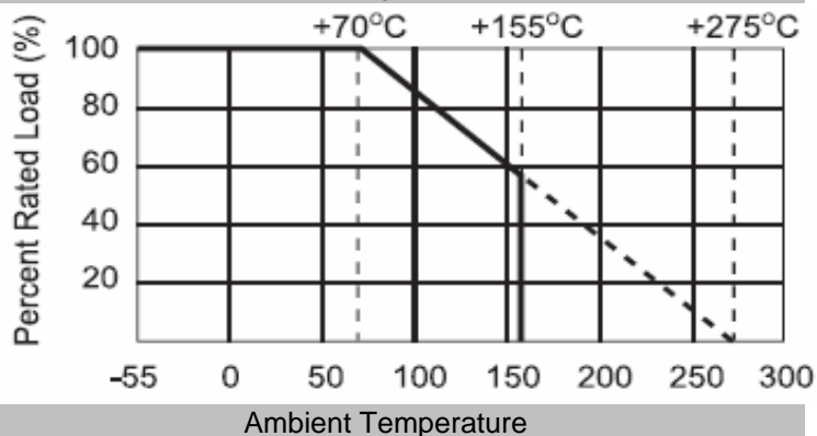
Derating Curve
