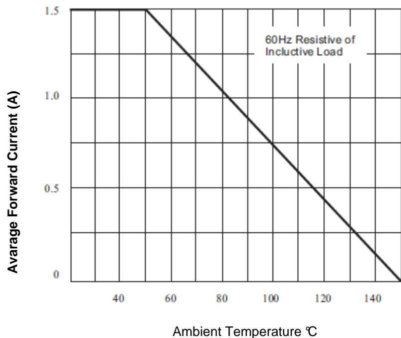
Derating Curve for Output Rectified Current
