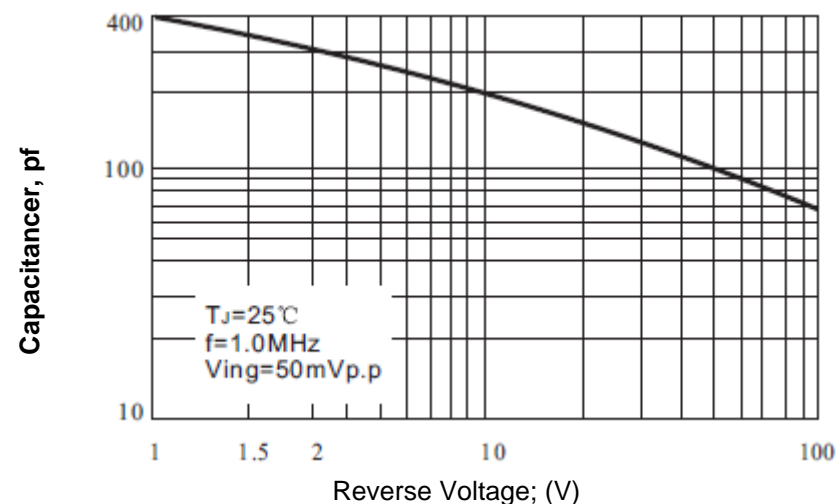
Typical Junction Capacitance per Leg
