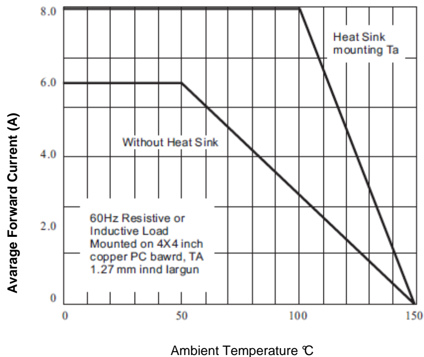
Typical Forward Current Characteristics Derating Curve
