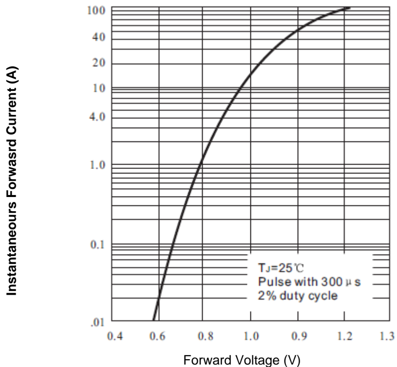
Typical Forward Characteristics
