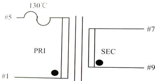
Single Output
