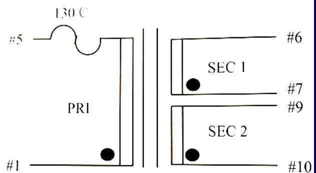
Dual Output
