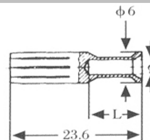
Female Contact
