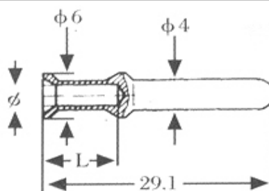
Male Contact
