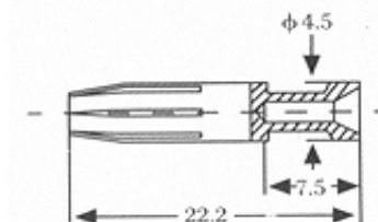
Female Contact
