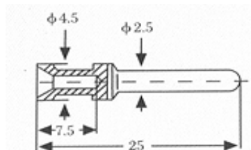
Male Contact
