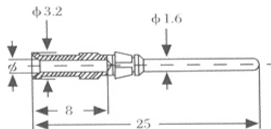
Male Contact
