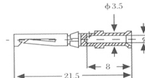
Female Contact
