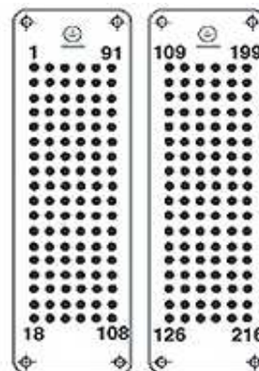
Contact arrangement view from termination side
