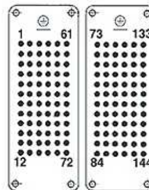
Contact arrangement view from termination side
