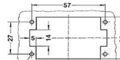
Panel cut out
