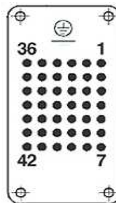
Contact arrangement view from termination side
