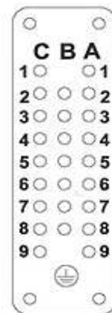
Contact arrangement view from termination side
