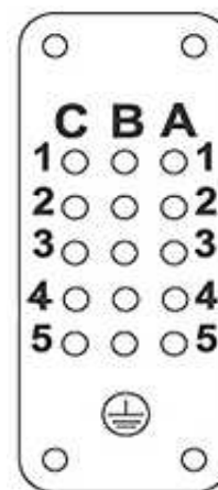
Contact arrangement view from termination side
