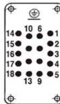
Contact arrangement view from termination side
