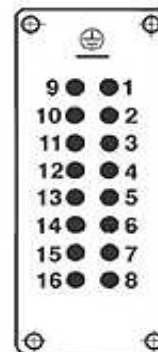
Contact arrangement view from termination side
