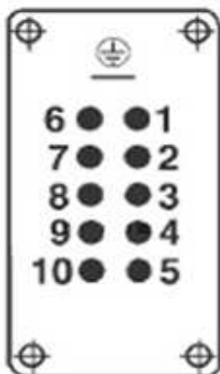
Contact arrangement view from termination side
