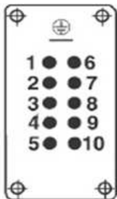
Contact arrangement view from termination side
