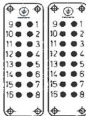
Contact arrangement view from termination side
