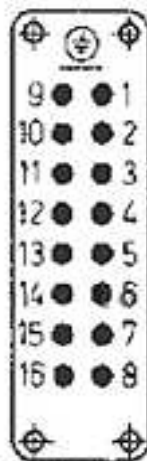
接插针排序 Contacts arrangement view from termination side
