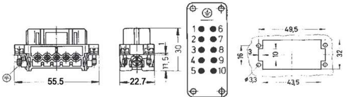
Panel cut out for inserts for use without Hoods/housings
